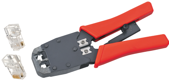
HT-500R - Ratchet modular crimping tool
