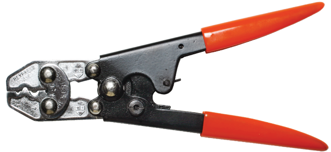
HEXA6-10 - Ratchet indent crimping tool for copper lugs and ferrules
